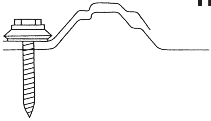
ROOFING - EAVE AND END LAPS
